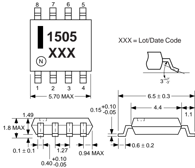
UPB1505GR PACKAGE OUTLINE G08
