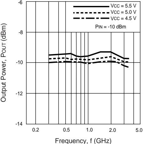
OUTPUT POWER vs. INPUT FREQUENCY AND SUPPLY VOLTAGE AT +85^\circ\text{C}
