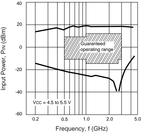
INPUT POWER vs. INPUT FREQUENCY
