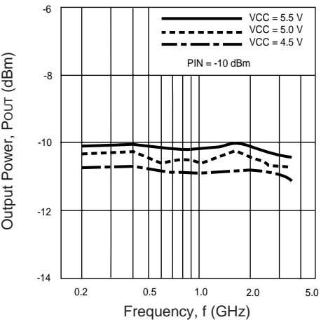
OUTPUT POWER vs. INPUT FREQUENCY AND SUPPLY VOLTAGE
